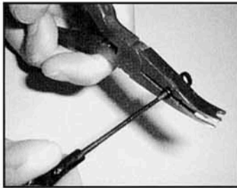
▲ USE THE LARGE HOLE TO HOLD THE BALL LINK WHILE MAKING ADJUSTMENTS.
