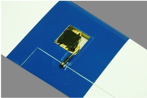
AILERON SERVO MOUNTING
