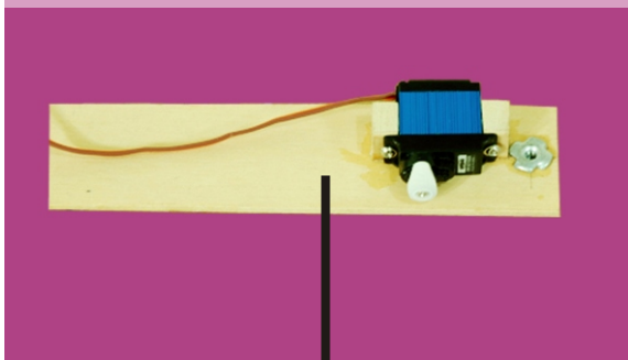
ELEVATOR SERVO MOUNTING (V.1)
